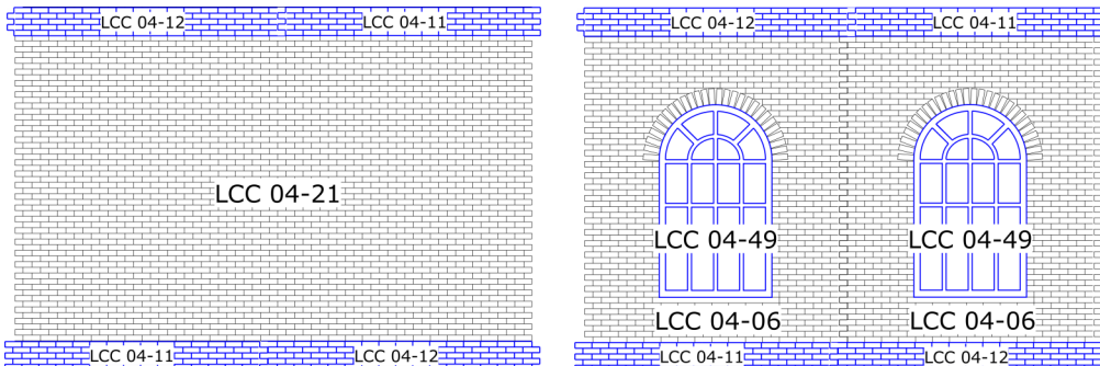
FRONT AND BACK ELEVATIONS
