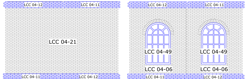
FRONT AND BACK ELEVATIONS
